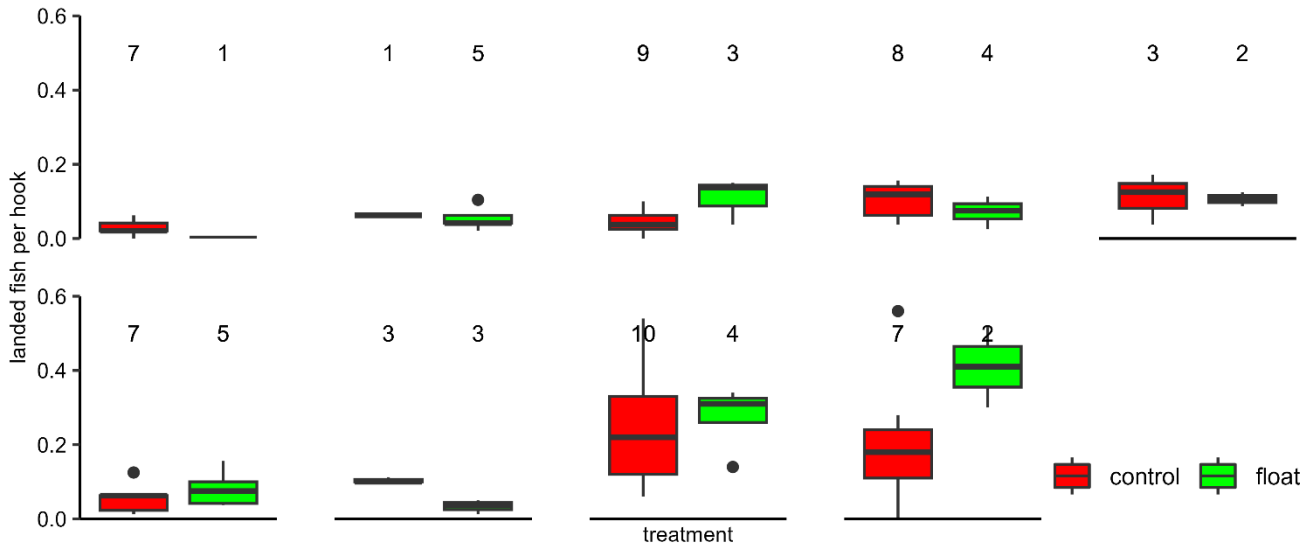
Figure 7. Catches of all landed fish from Vessel B, by line and treatment (control vs modified floats). Numbers above boxes show number of line sections in each treatment.
